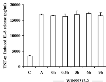
Fig. 6. Effect of WIN55212-2 on IL-8 release in TNF- \alpha pre-stimulated HT-29 cells. Confluent monolayers of cells were activated with TNF- \alpha (100 ng/ml) and WIN55212-2 ( 10^{-6} M) added at the time points indicated post-activation. Supernatants were collected 24 h after TNF- \alpha activation and analyzed by ELISA for IL-8. Data represent means \pm S.E.M. of three separate experiments.
