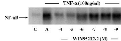
Fig. 7. Effect of WIN55212-2 on TNF- \alpha induced NF- \kappa B activation in HT-29 cells. Nuclear extracts were prepared from confluent cultures pre-treated for 2 h with WIN55212-2 prior to activation with TNF- \alpha (100 ng/ml) for 1 h. Nuclear proteins were probed with ^{32} P labeled \kappa B oligomer and autoradiographed. C: non-activated control; A: TNF- \alpha activated control. The blot is representative of three separate experiments.
