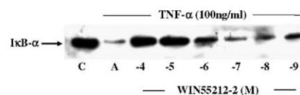
Fig. 8. Effect of WIN55212-2 on TNF- \alpha induced I \kappa B degradation in HT-29 cells. Cell lysates were prepared from cultures pre-treated with WIN55212-2 for 2 h prior to activation with TNF- \alpha (100 ng/ml) for 30 min. Levels of I \kappa B were determined by Western blotting using a specific monoclonal antibody as described in methods. C: non-activated control; A: TNF- \alpha activated control. The blot is representative of three separate experiments.
