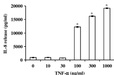
Fig. 1. TNF- \alpha induced release of IL-8 from HT-29 cells. Confluent monolayers of cells were stimulated with increasing concentrations of TNF- \alpha (10–1000 ng/ml) for 24 h. IL-8 release was measured by ELISA as described in methods. Data represent means \pm S.E.M. of three separate experiments. * P < 0.01.
